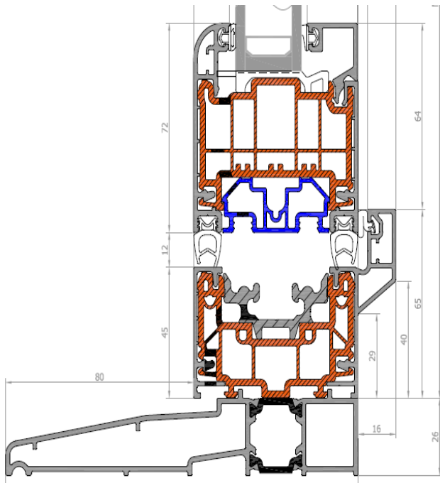
OPEN OUT WITH SILL
